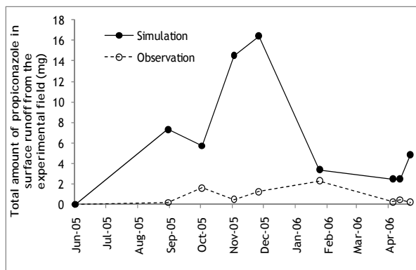
Figure 33. Calibrated values for the total amount of propiconazole in surface runoff from Bjørnebekk, 2005-2006
