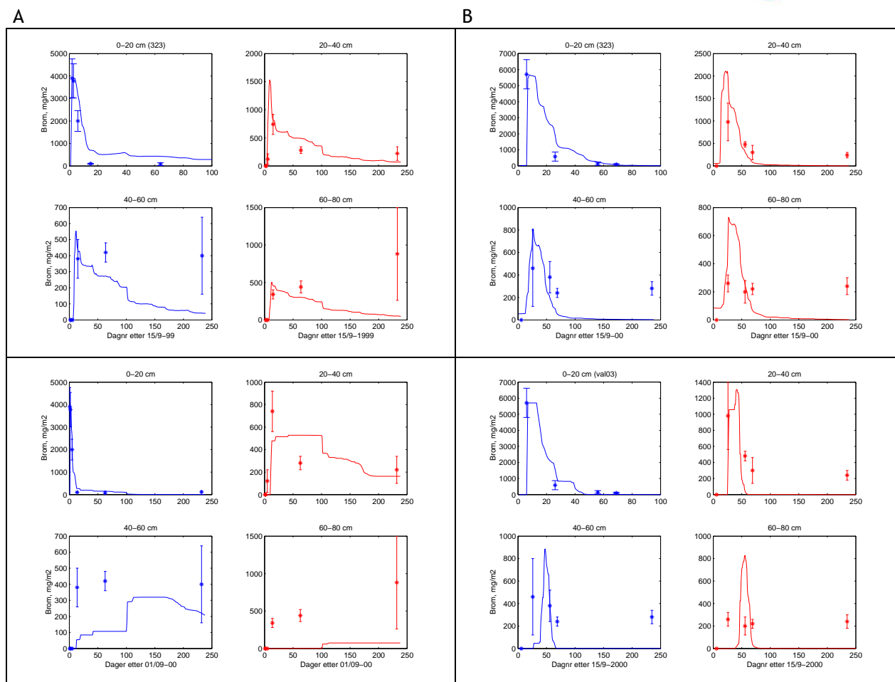
Figure 18. Measured and simulated values for bromide in soil at Rustad, 1999/2000 and 2000/2001. Simulated with MACRO and PRZM.
